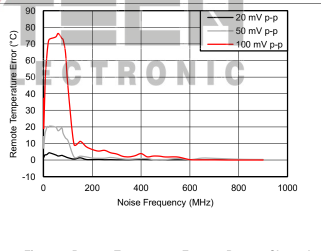
Figure 7. Remote Temperature Error vs Remote Channel Noise Frequency
